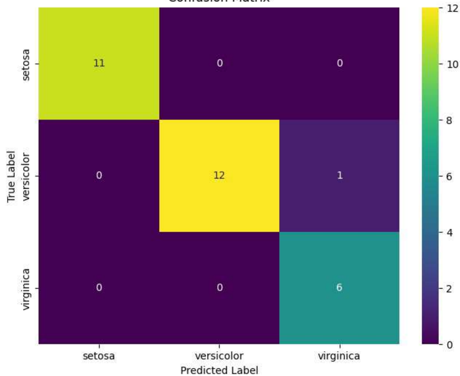
Confusion Matrix
