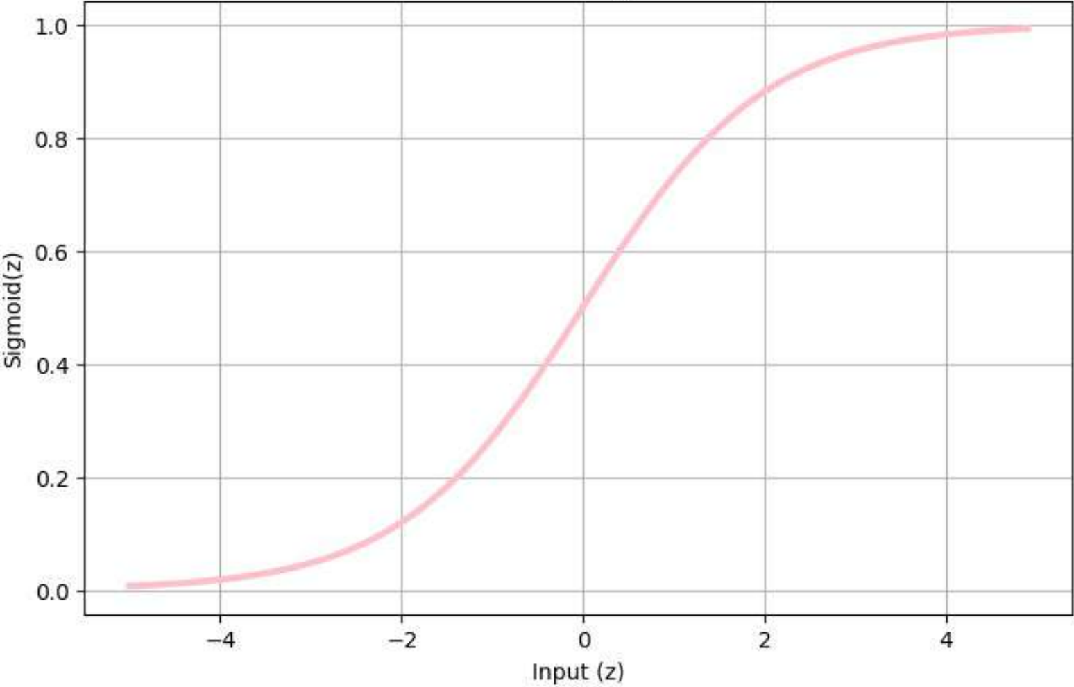
Visualization of the Sigmoid Function
