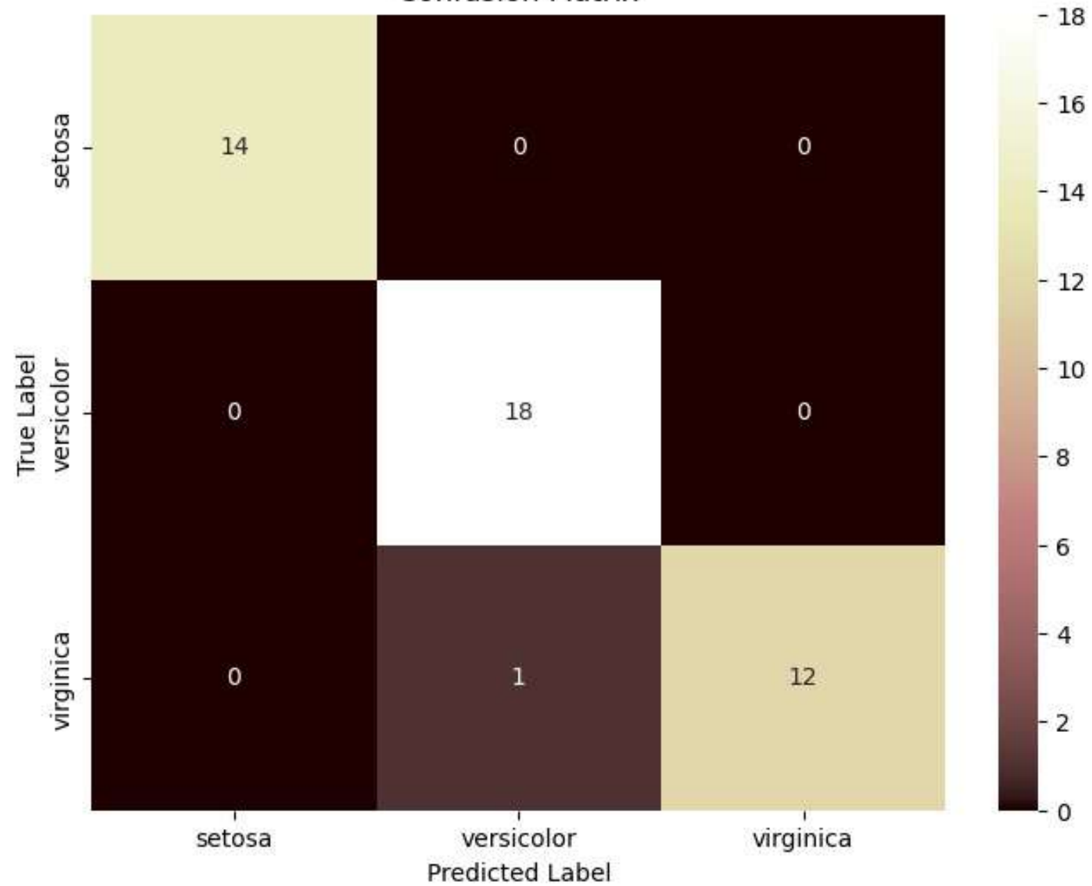
Confusion Matrix
