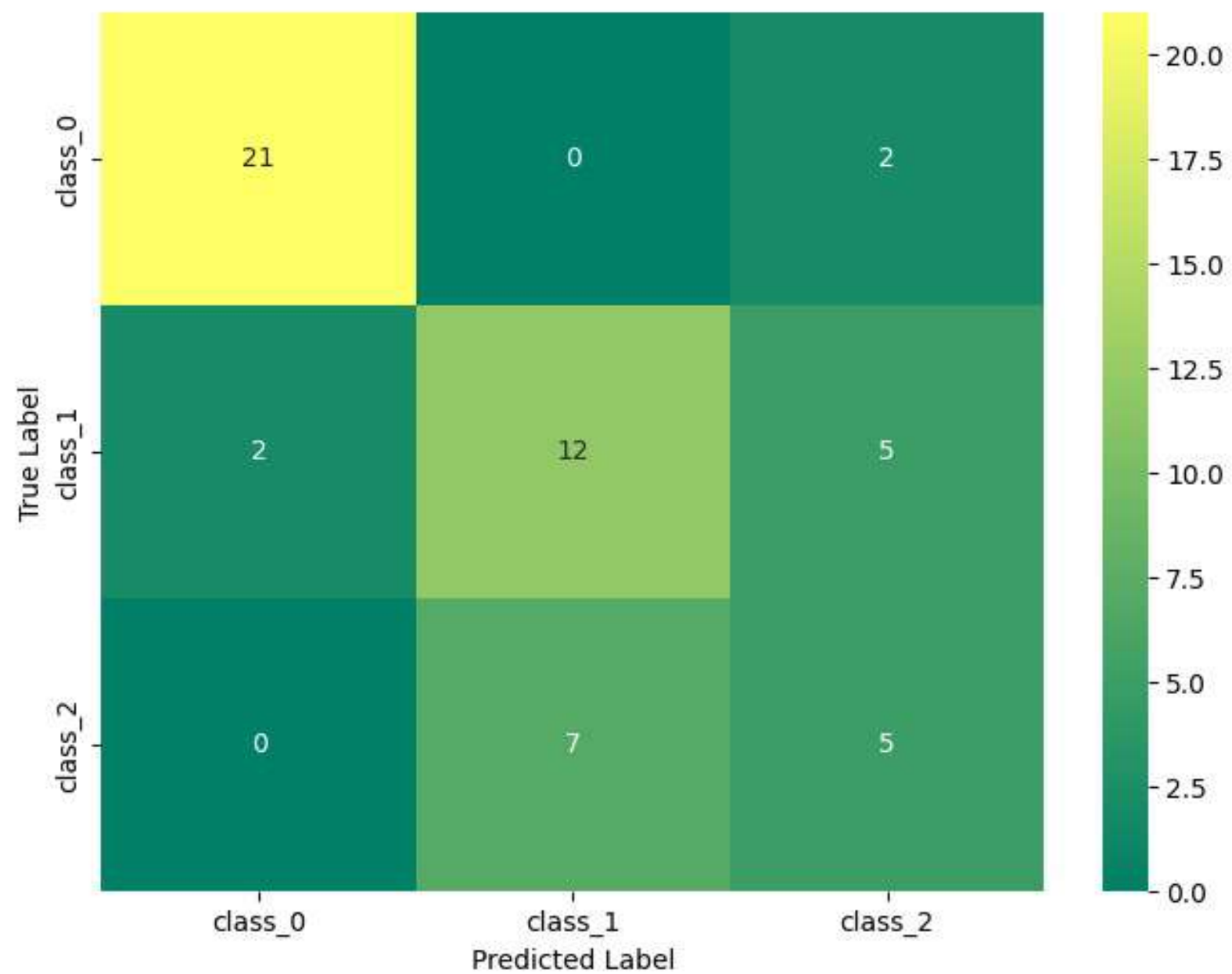
Confusion Matrix
