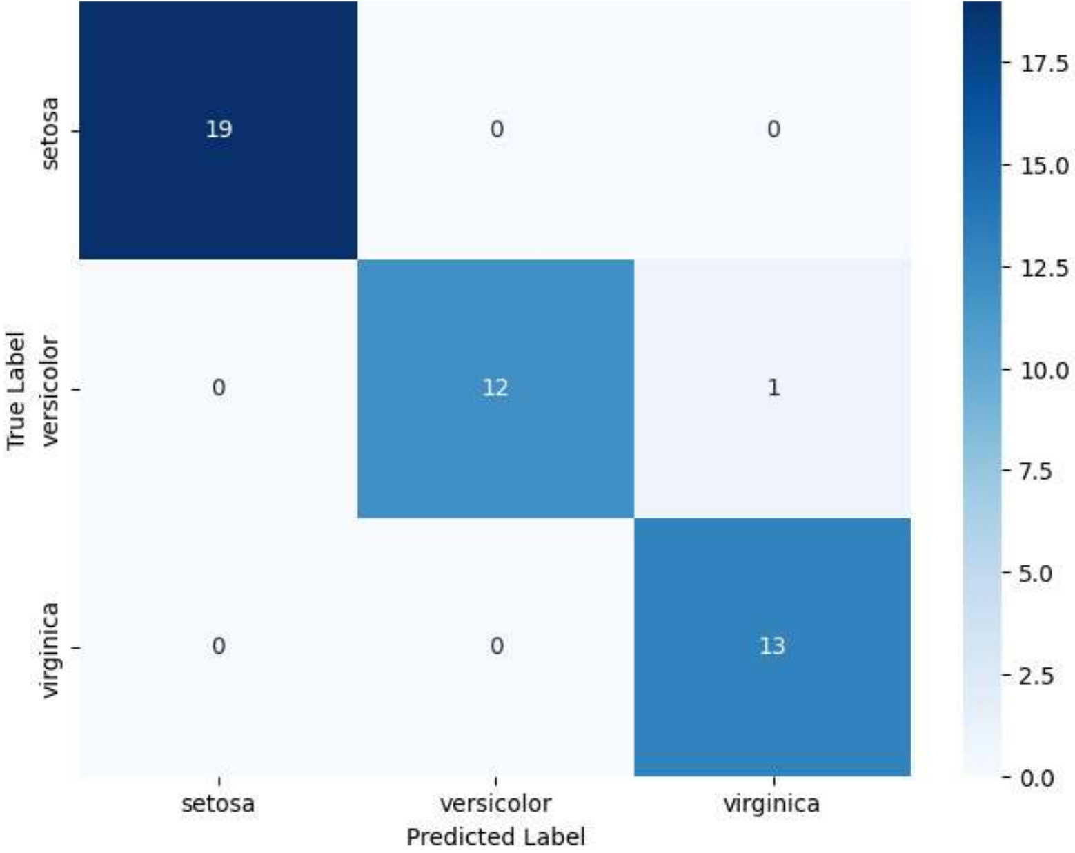
Confusion Matrix
